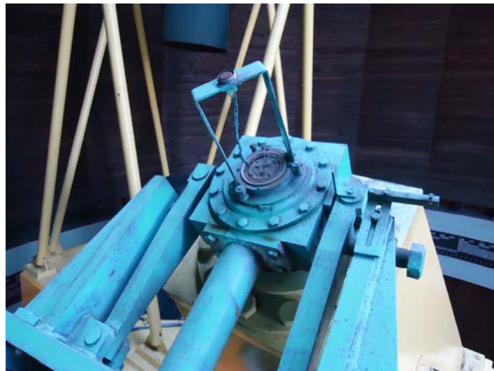
Figure 14. Detail of right ascension axis mechanism and resolver. 19-poles M-23 female connector (top).
