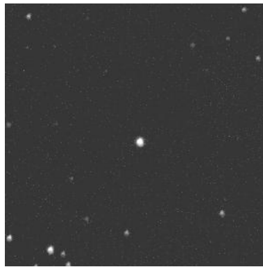
Figure 1. CCD field subframe from the 1.65 m telescope with GD358 (in the center). Night of May 17.
