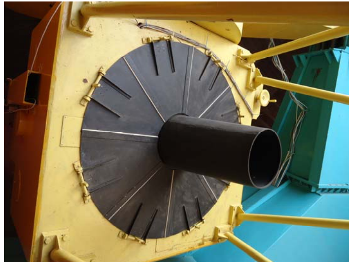
Figure 13. Detail of opening doors -protective covers of the primary mirror.
