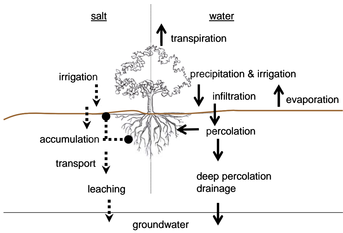
Figure 2. Schematic of water and salt balance in an irrigated crop. Solid arrows represent water movement and dashed arrows, salts.
