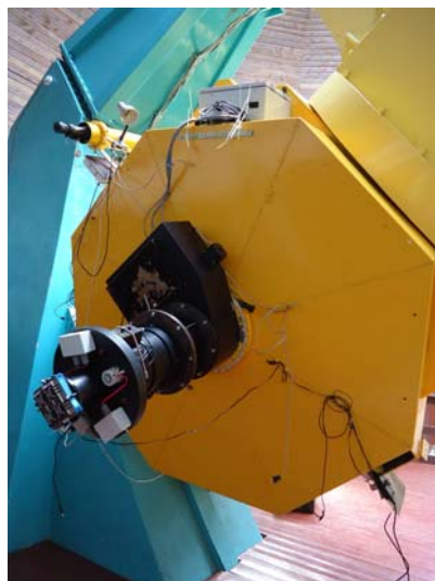
Figure 18. Detail of the telescope: from bottom to top, Apogee CCD Camera, focal reducer, filter wheel, focal reducer, autogiding system and derotator.
